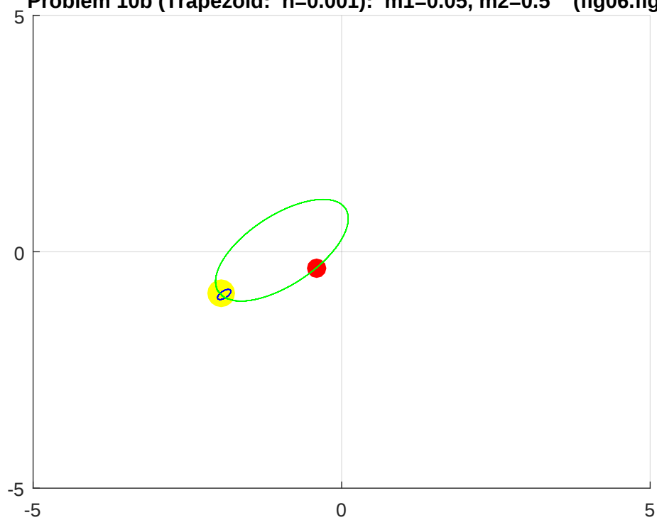
Celestial Mechanics: Two (2) Body Problem Problem 10b (Trapezoid: h=0.001 ): m_1=0.05 , m_2=0.5 (fig06.fig)
